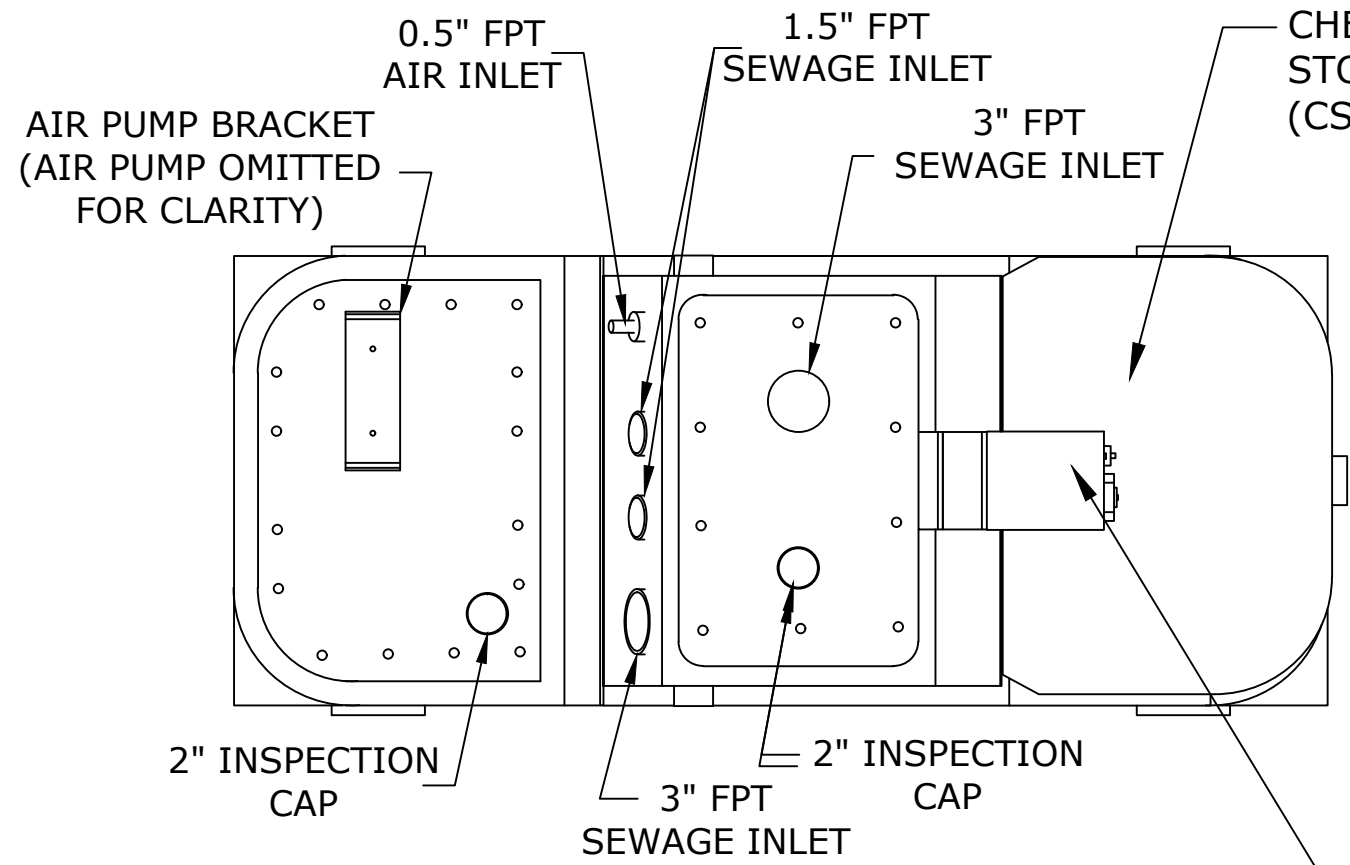
TOP CHEMICAL INJECTION METERING PUMP (CIMP)
